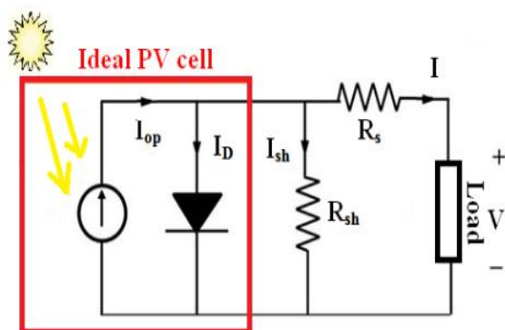
Fig. 1: An equivalent circuit of the PV.
