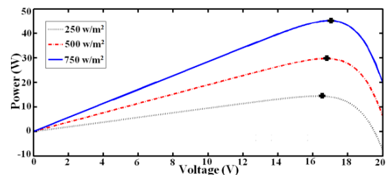
Fig. 2: Relationship between output voltage and power of the PV cell under different irradiation conditions
