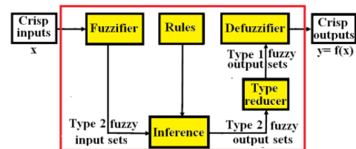
Fig. 3: Type 2 fuzzy inference system structure
