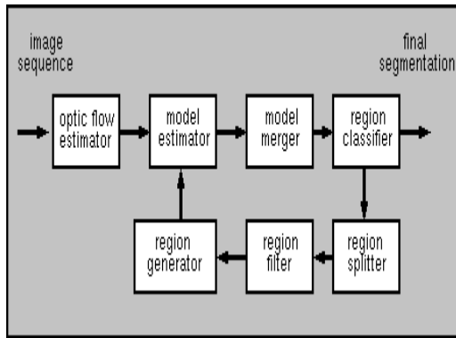
Figure 4: Region Based Image Segmentation
