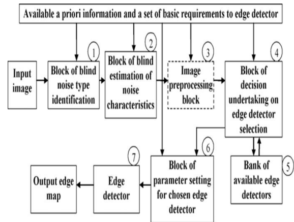
Figure 5: Block Diagram for Edge Detector
