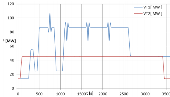
Fig. 4. Comparison of generation from wind turbines with gusts of wind and slight breeze.
