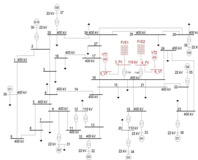
Fig. 1: The initial scheme of IEEE39 Bus System with implemented renewable energy sources (wind generators and photovoltaic invertors).
