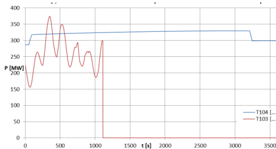
Fig. 5. Outage of transformer T103 due to overload.
