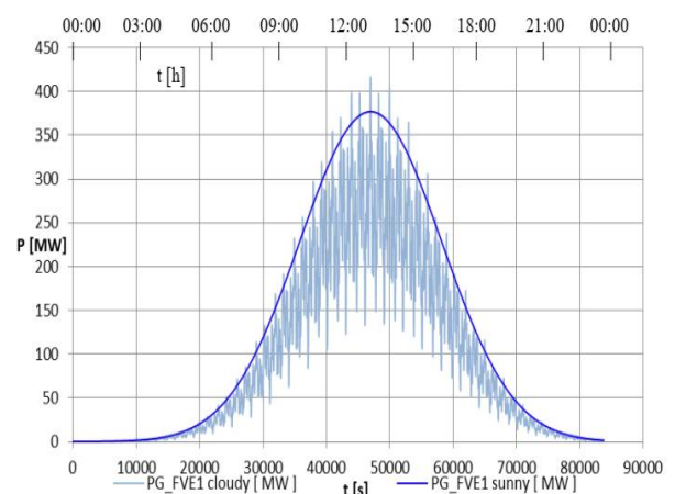
Fig. 3. Comparison of generation from PV during cloudy (FVE1) and sunny days (FVE2).
