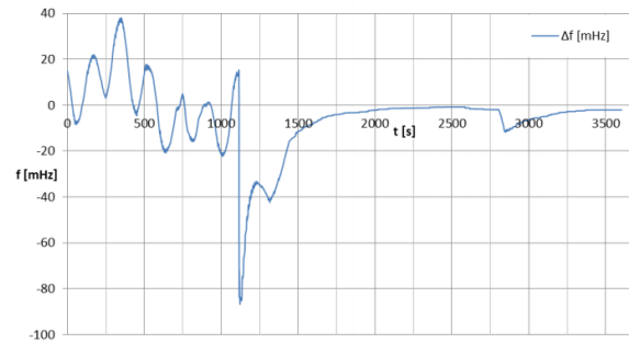
Fig.6 Frequency deviation during the outage of transformer.
