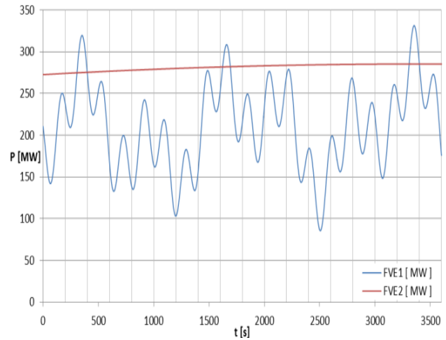
Fig. 2. Comparison of generation from PV during cloudy (FVE1) and sunny days (FVE2).
