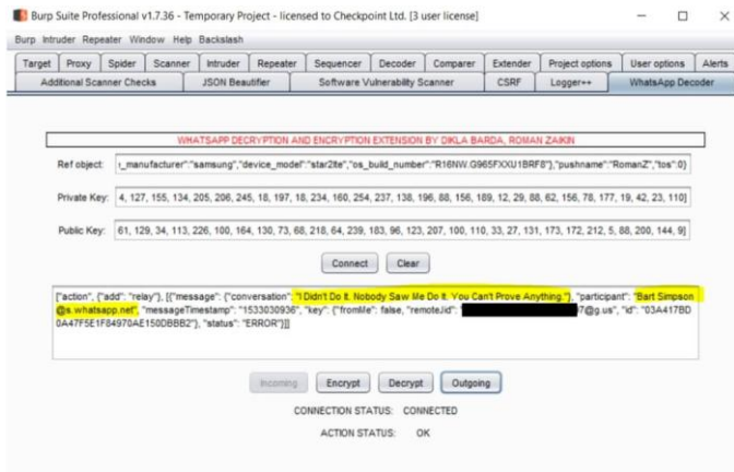
Fig 7.Screat Password
