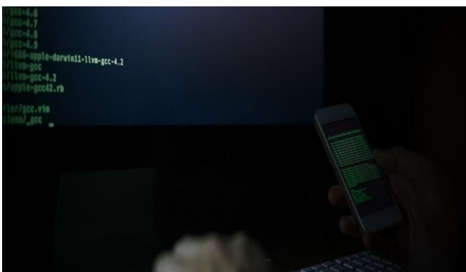
Fig 2.Hacking Coding
