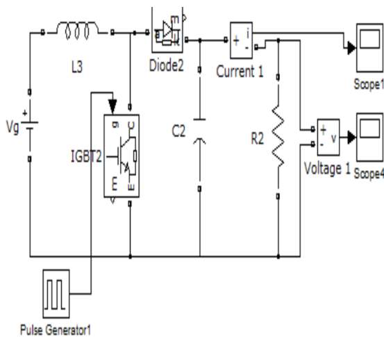
Figure.3: Boost converter
